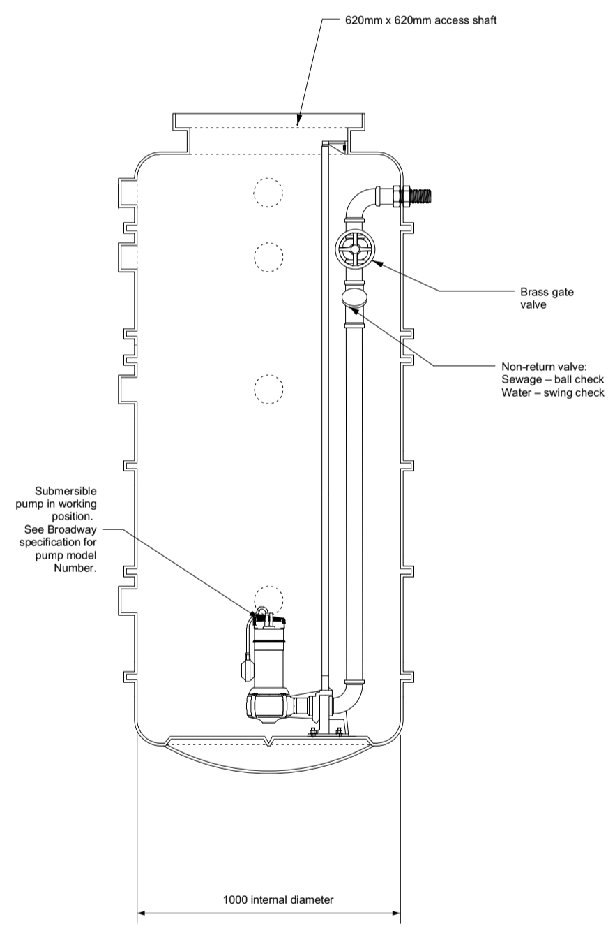
SECTIONAL ELEVATION
