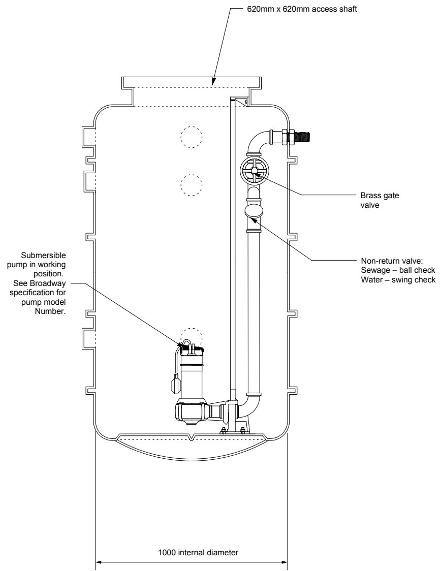
SECTIONAL ELEVATION
