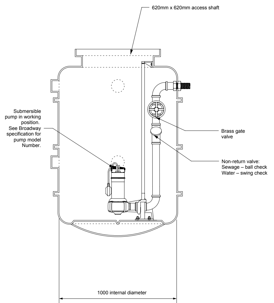
SECTIONAL ELEVATION
