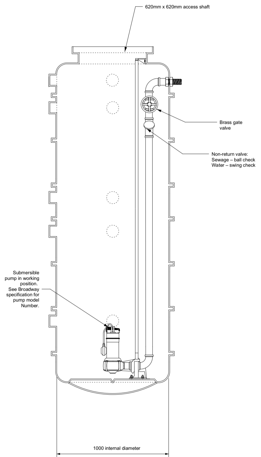
SECTIONAL ELEVATION
