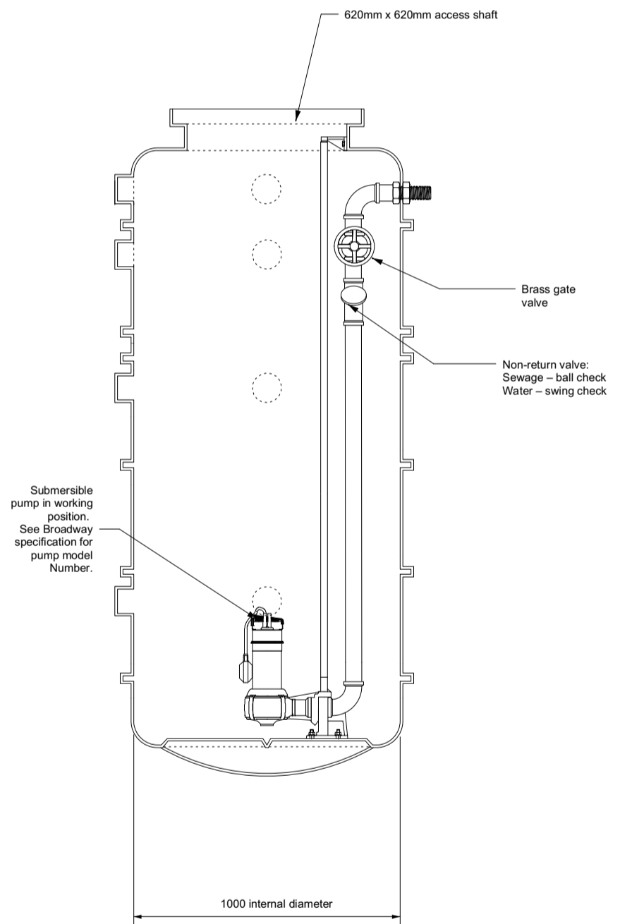
SECTIONAL ELEVATION
