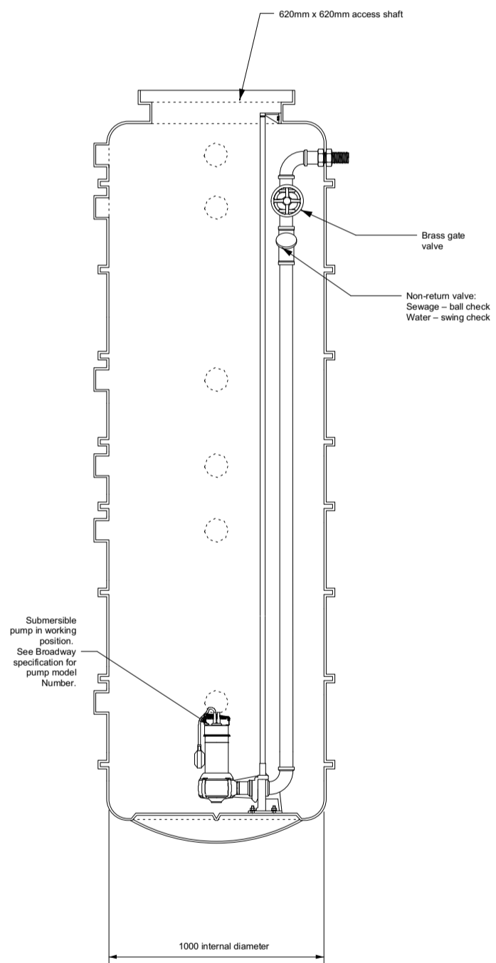
SECTIONAL ELEVATION
